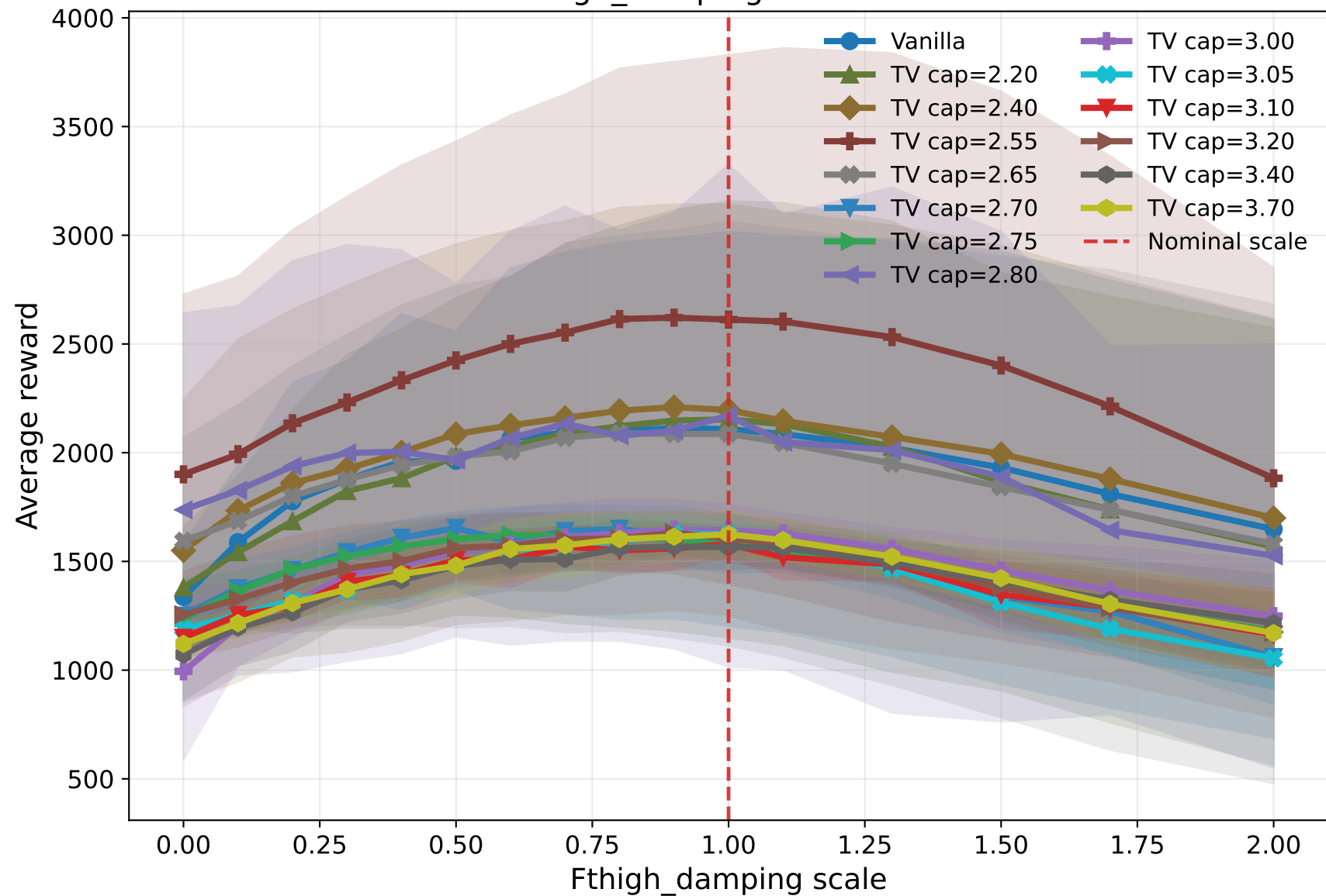
Fthigh_damping robustness
